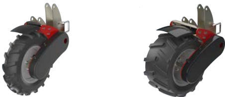
PAIR OF DRIVE WHEELS KIT MOD. S - DIM. Ø575x145 MM PAIR OF DRIVE WHEELS KIT MOD. M - DIM. Ø570X270 MM
